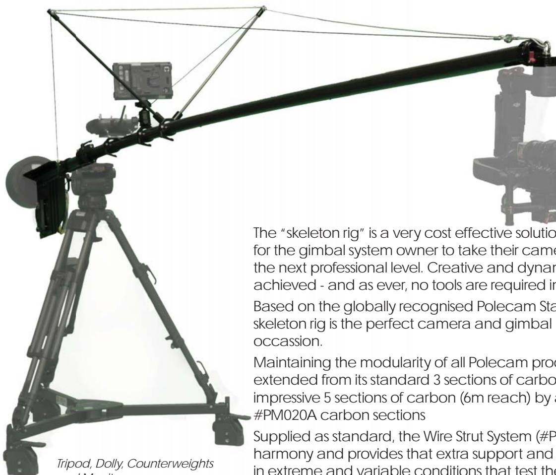
Skeleton rig at 3 sections (3.5m reach) with Ronin M shown with the Toshiba IK-4K and Fujinon Xt17 zoom lens (not included)
